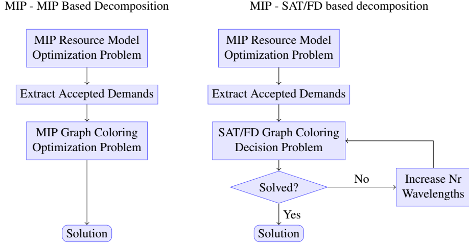
Fig. 1. Solution Approach
