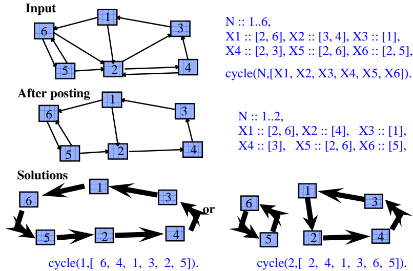
Figure 3: example of the cycle constraint
