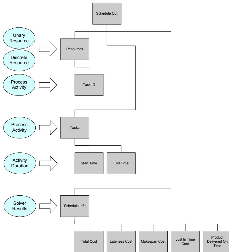
Fig. 9. Scheduling Results into the Translational Model.
