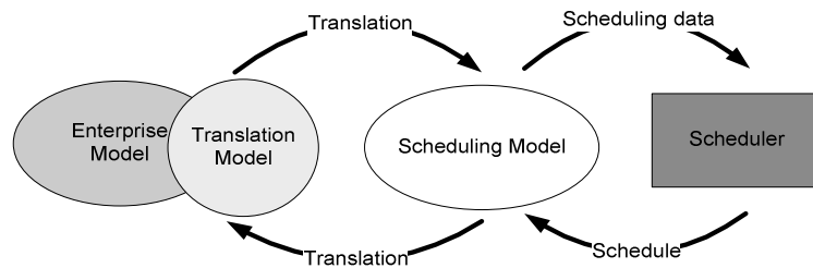
Fig. 1. Integration Architecture between Enterprise Model and Scheduling model.
