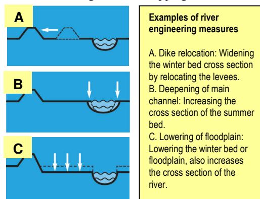
Figure 1. River engineering measures
